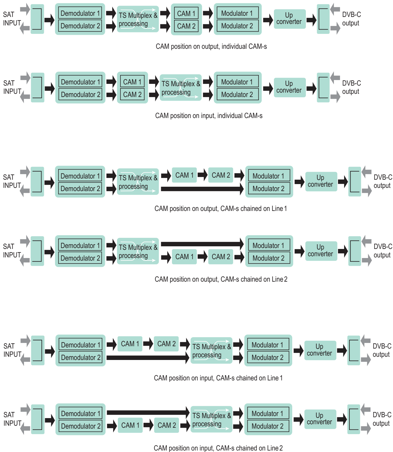
Figure 32. CAM configuration
