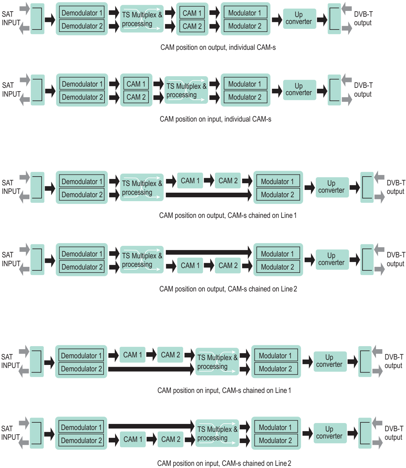
Figure 32. CAM configuration
