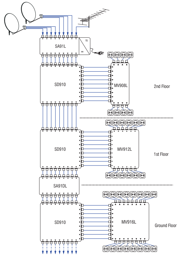
Figure 1. Floor by floor installation powered from SA91L.
