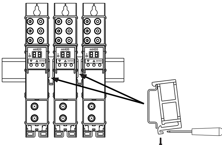
Figure 6. Mounting or removing to/from DIN rail of plastic spacers (supplied).
